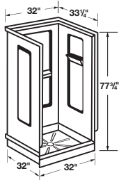
Shown with Shower Floor
