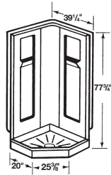
Shown with Shower Floor
