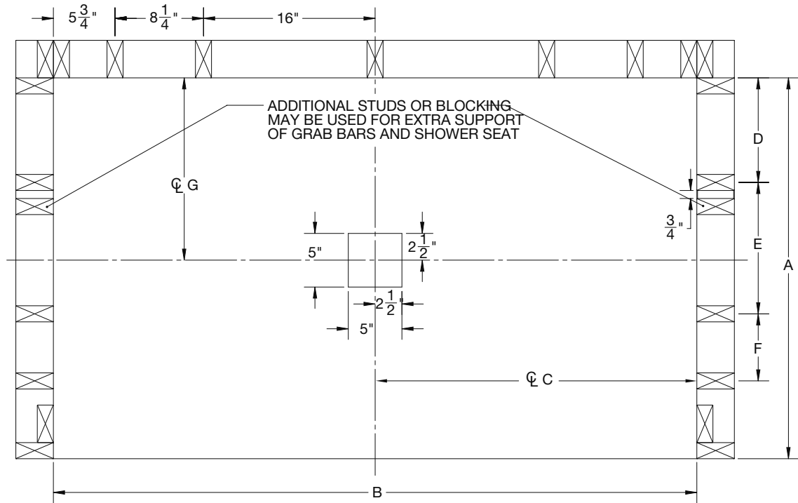
ROUGH-IN "PLAN VIEW"
